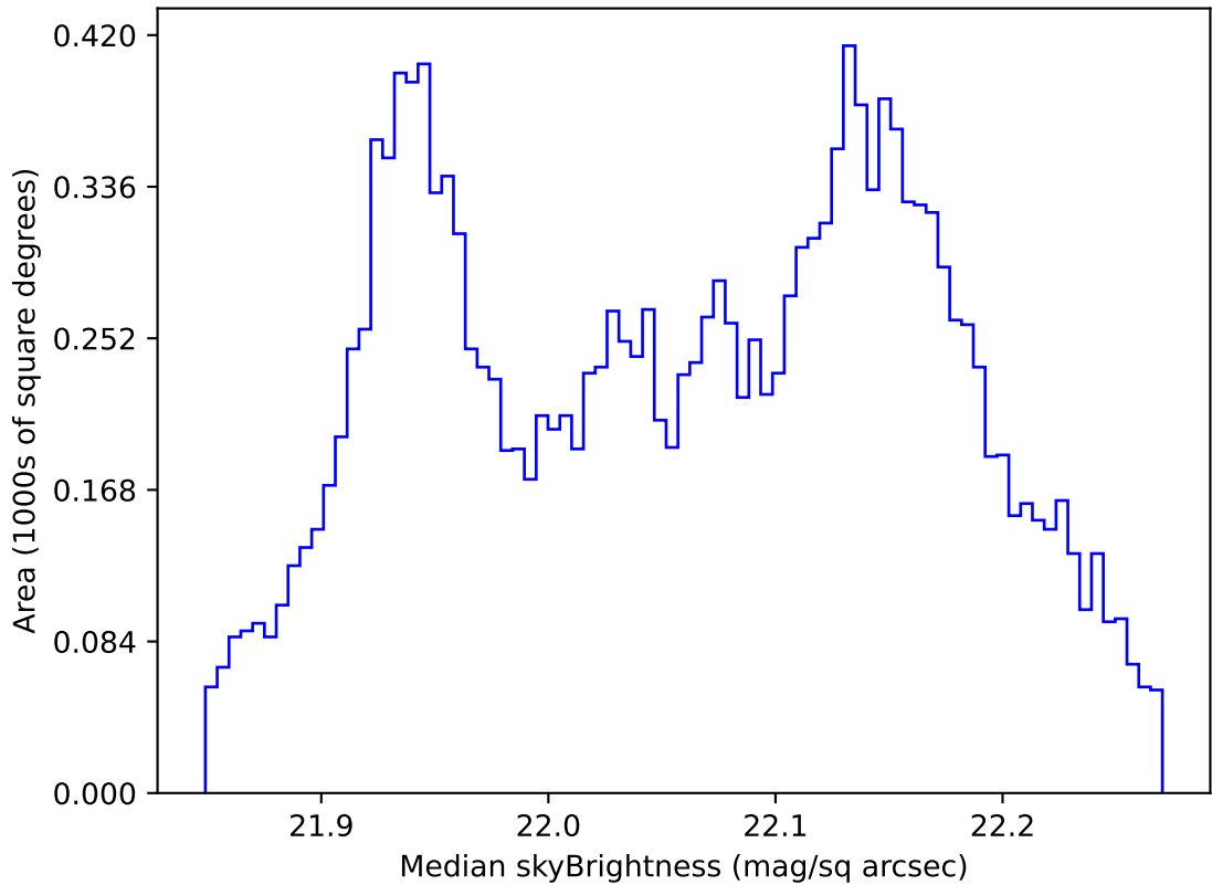
too_elab_2yr_r128_d3_ugrizy_v3.4_10yrs WFD g band: Median skyBrightness
