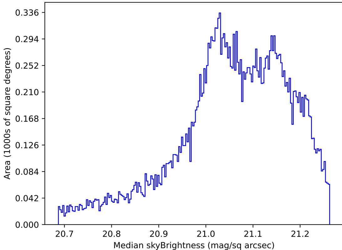
too_elab_2yr_r128_d3_ugrizy_v3.4_10yrs All sky r band: Median skyBrightness
