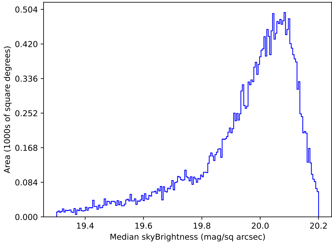
too_elab_2yr_r128_d3_ugrizy_v3.4_10yrs All sky i band: Median skyBrightness
