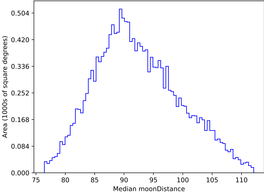
too_elab_2yr_r128_d3_ugrizy_v3.4_10yrs WFD i band: Median moonDistance
