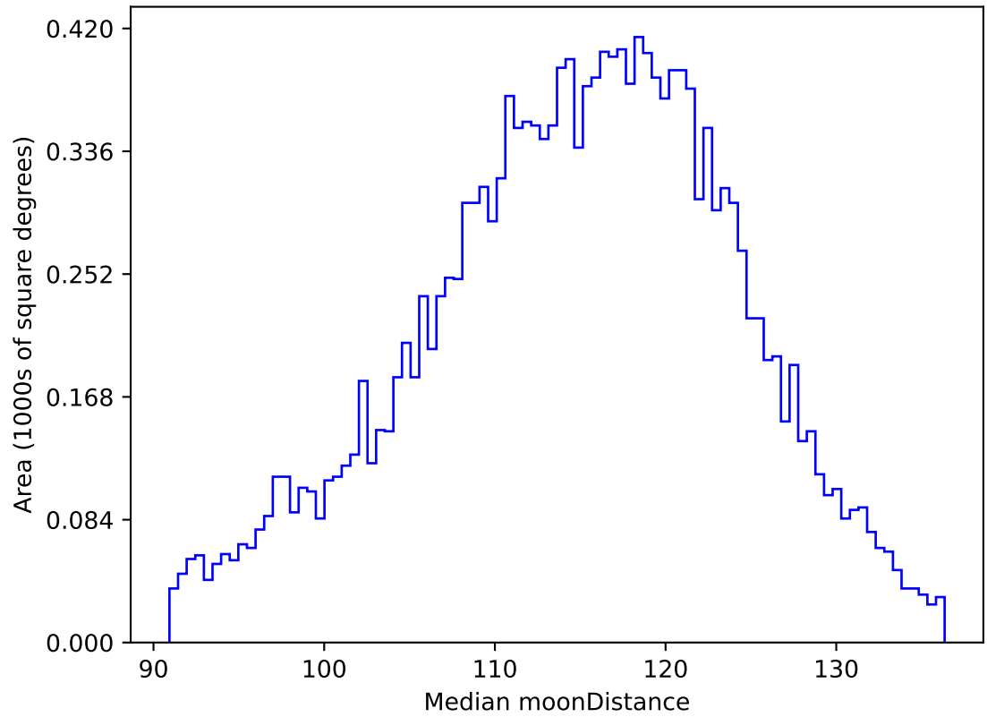
too_elab_2yr_r128_d3_ugrizy_v3.4_10yrs WFD g band: Median moonDistance
