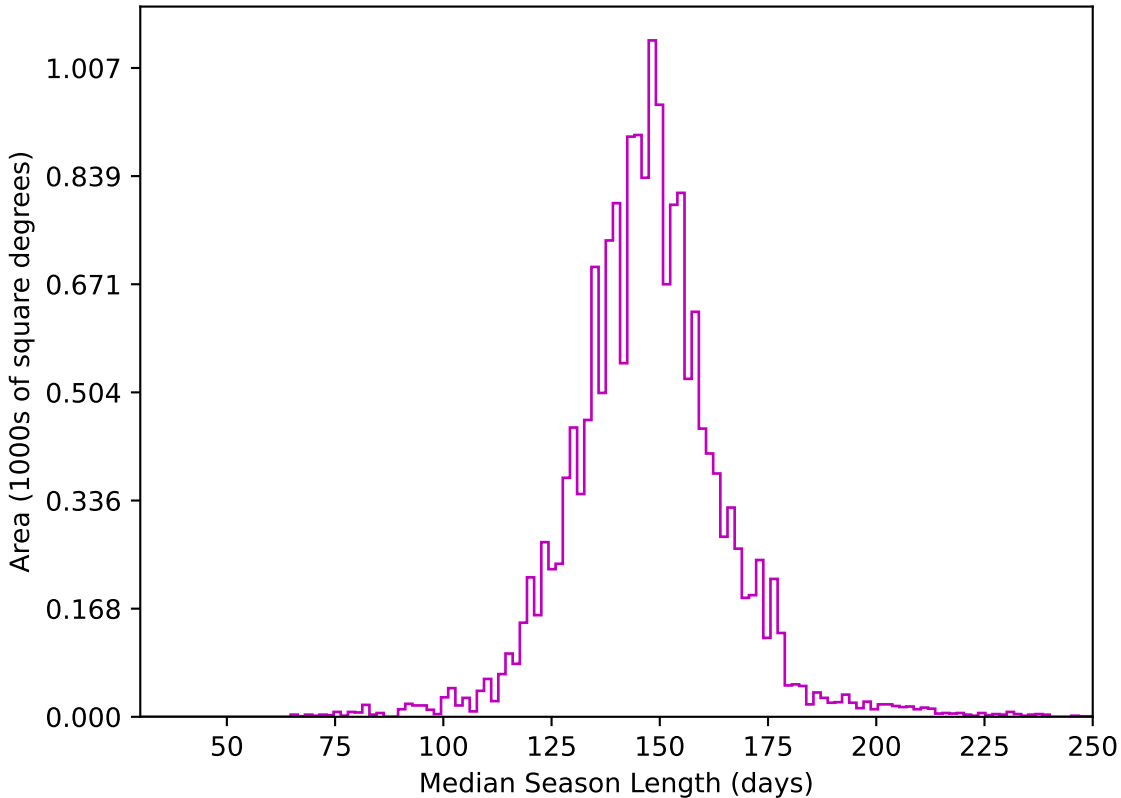
too_elab_2yr_r128_d3_ugrizy_v3.4_10yrs WFD z band: Median Season Length
