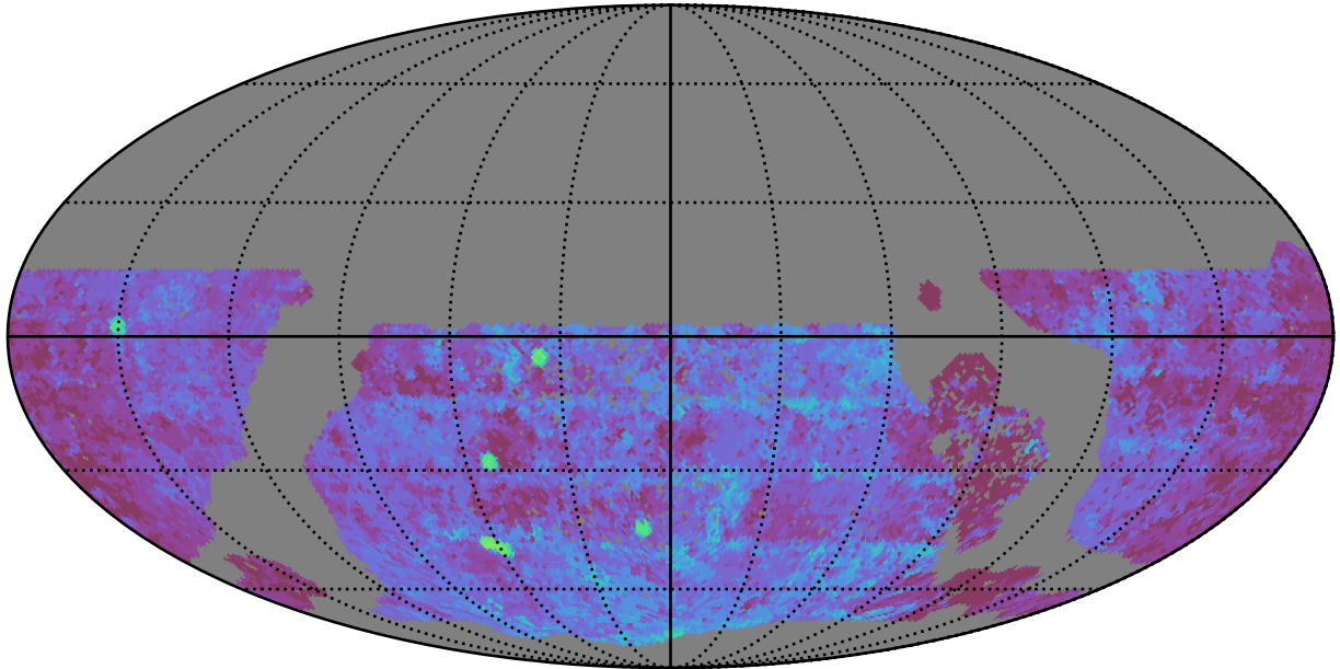
too_elab_2yr_r128_d3_ugrizy_v3.4_10yrs WFD u band: Median Season Length
