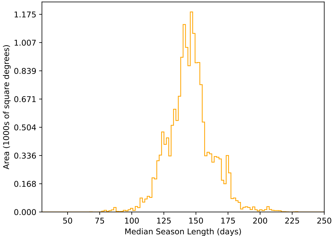
too_elab_2yr_r128_d3_ugrizy_v3.4_10yrs WFD r band: Median Season Length
