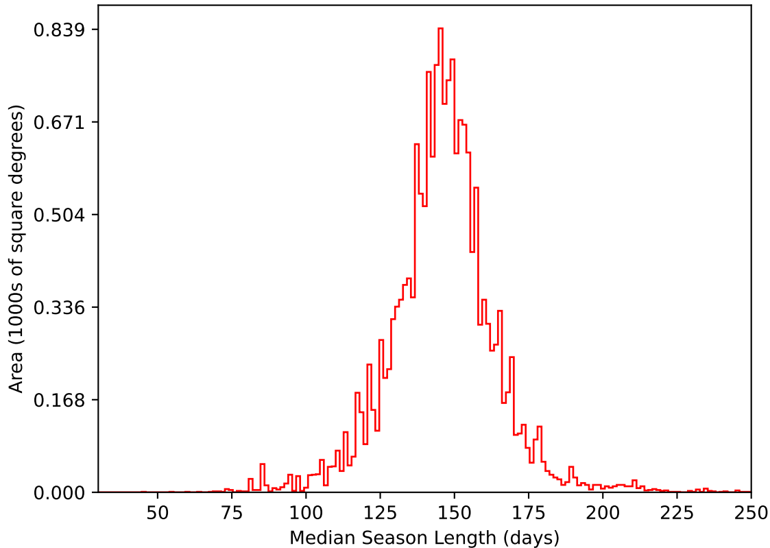
too_elab_2yr_r128_d3_ugrizy_v3.4_10yrs WFD i band: Median Season Length
