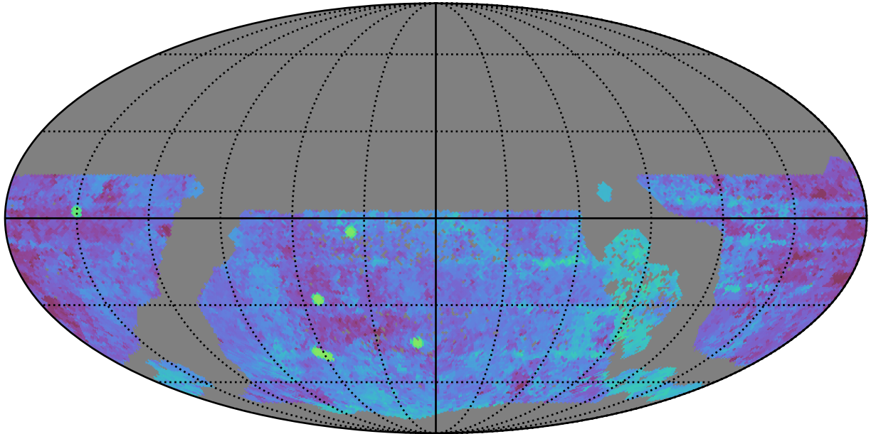
too_elab_2yr_r128_d3_ugrizy_v3.4_10yrs WFD g band: Median Season Length
