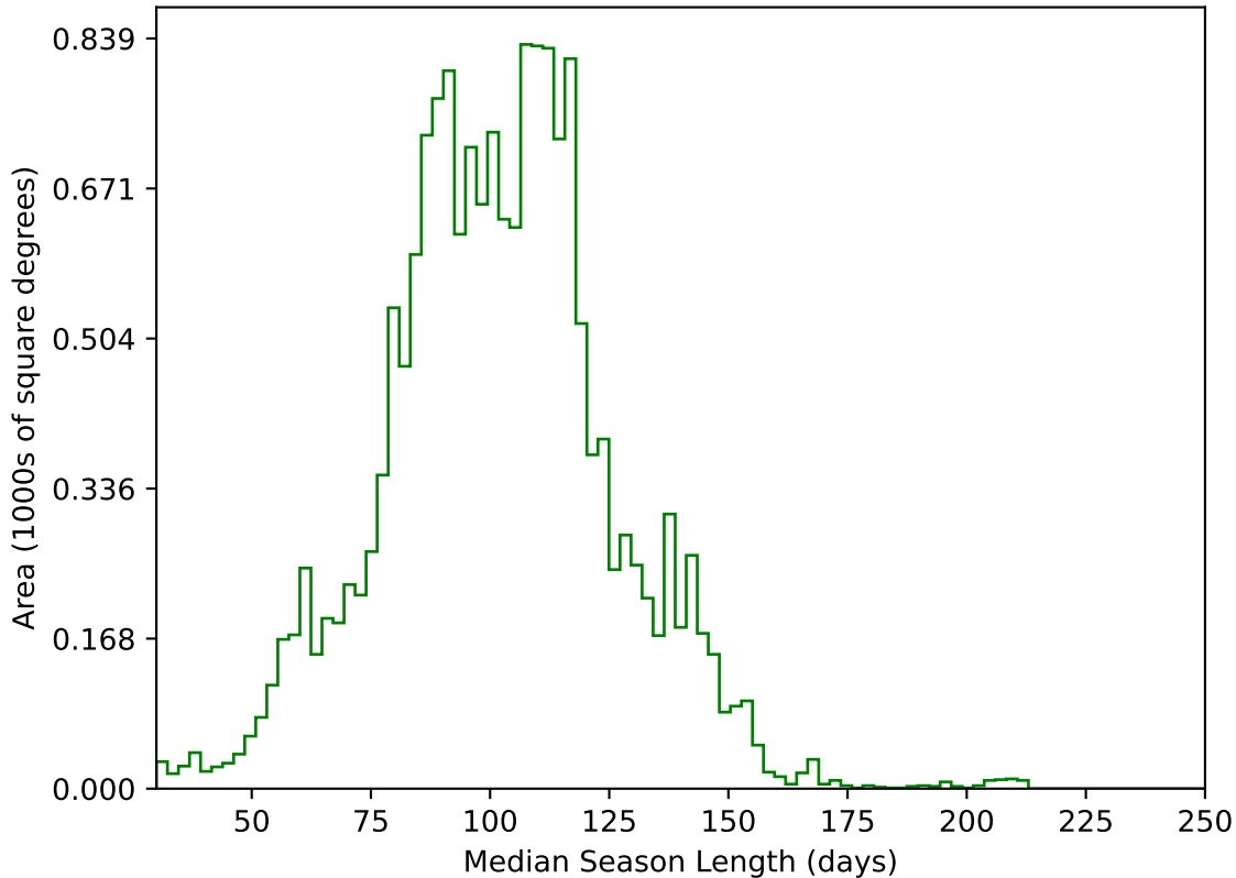
too_elab_2yr_r128_d3_ugrizyv3.4_10yrs WFD g band: Median Season Length
