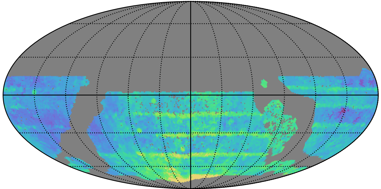
too_elab_2yr_r128_d3_ugrizy_v3.4_10yrs WFD all bands: Median Season Length
