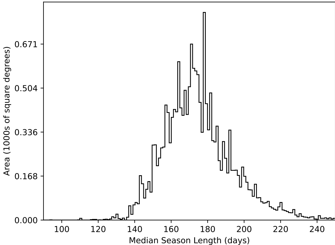
too_elab_2yr_r128_d3_ugrizy_v3.4_10yrs WFD all bands: Median Season Length
