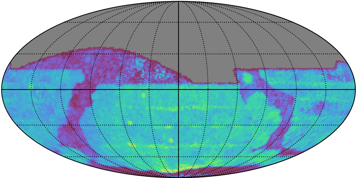
too_elab_2yr_r128_d3_ugrizy_v3.4_10yrs All sky z band: Median Season Length
