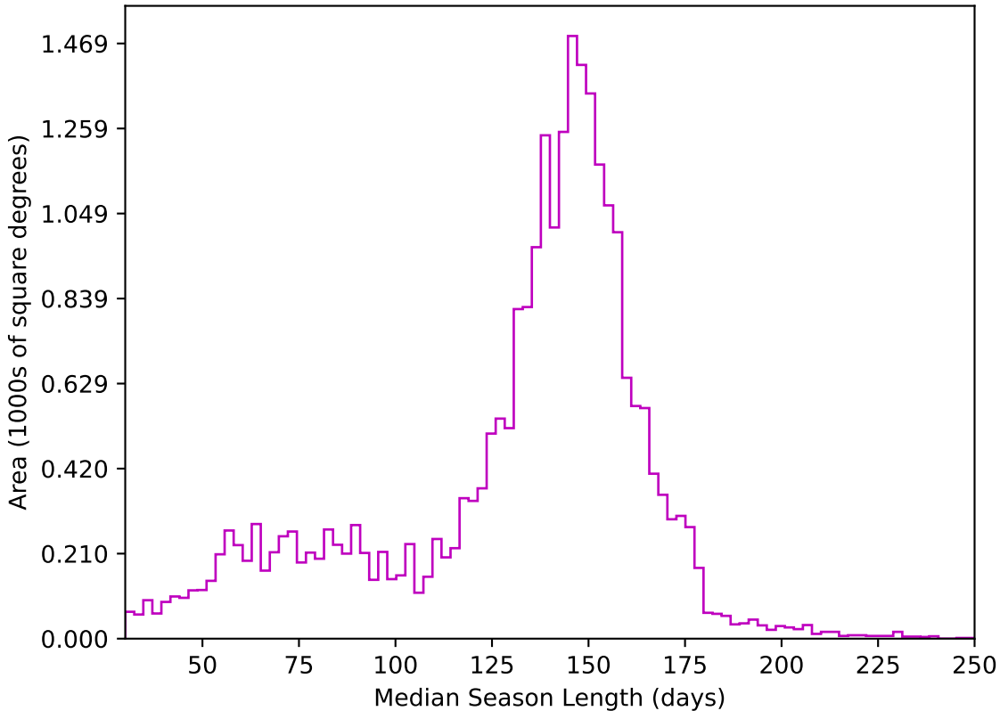
too_elab_2yr_r128_d3_ugrizy_v3.4_10yrs All sky z band: Median Season Length
