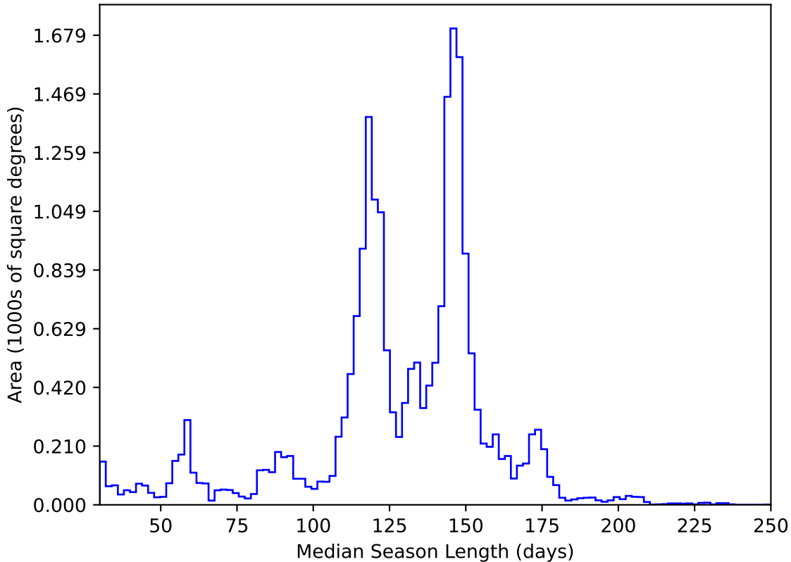
too_elab_2yr_r128_d3_ugrizy_v3.4_10yrs All sky y band: Median Season Length
