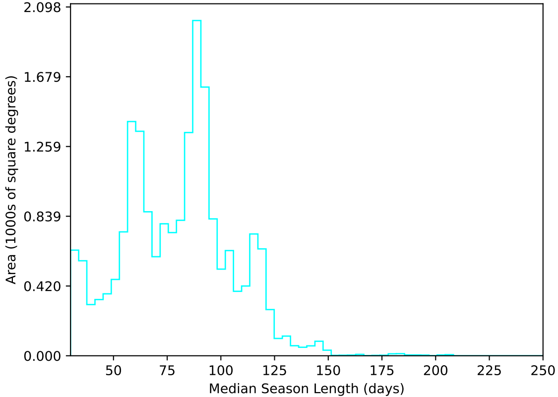
too_elab_2yr_r128_d3_ugrizyv3.4_10yrs All sky u band: Median Season Length
