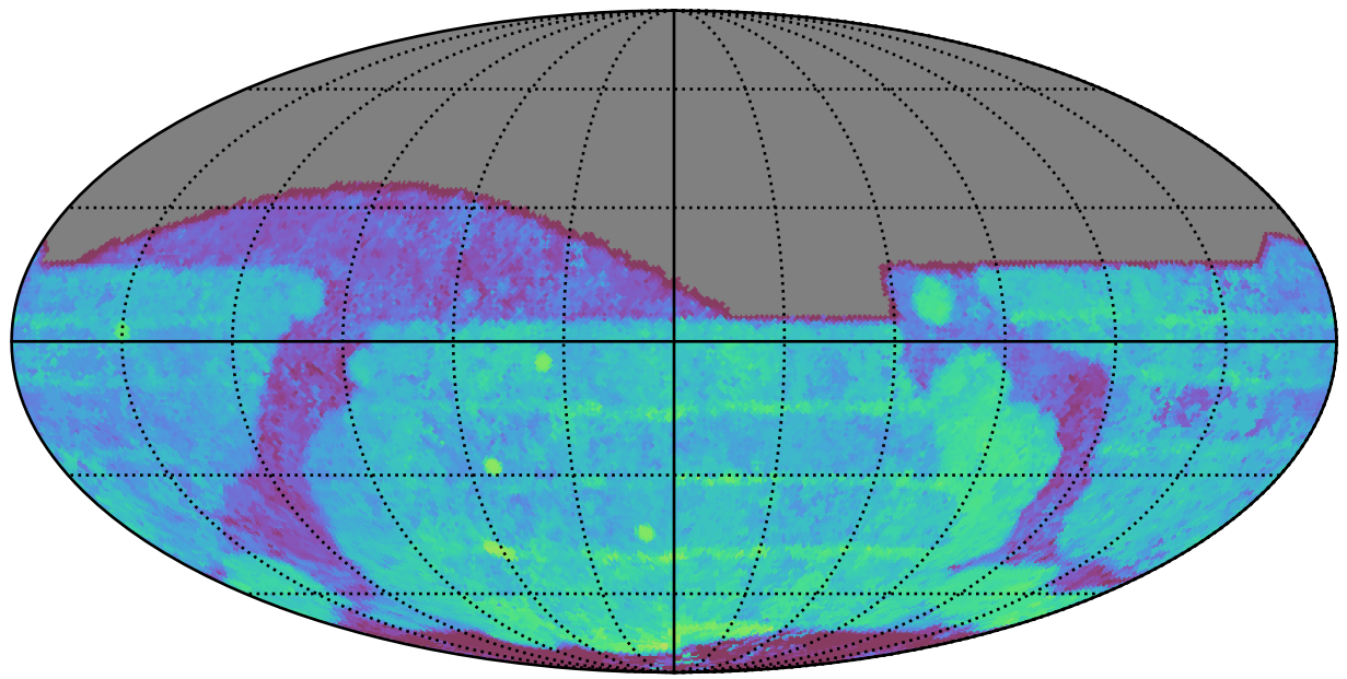
too_elab_2yr_r128_d3_ugrizy_v3.4_10yrs All sky r band: Median Season Length
