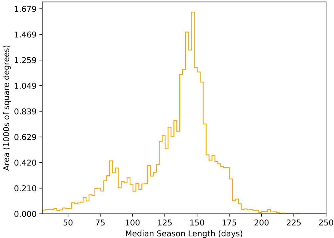
too_elab_2yr_r128_d3_ugrizy_v3.4_10yrs All sky r band: Median Season Length
