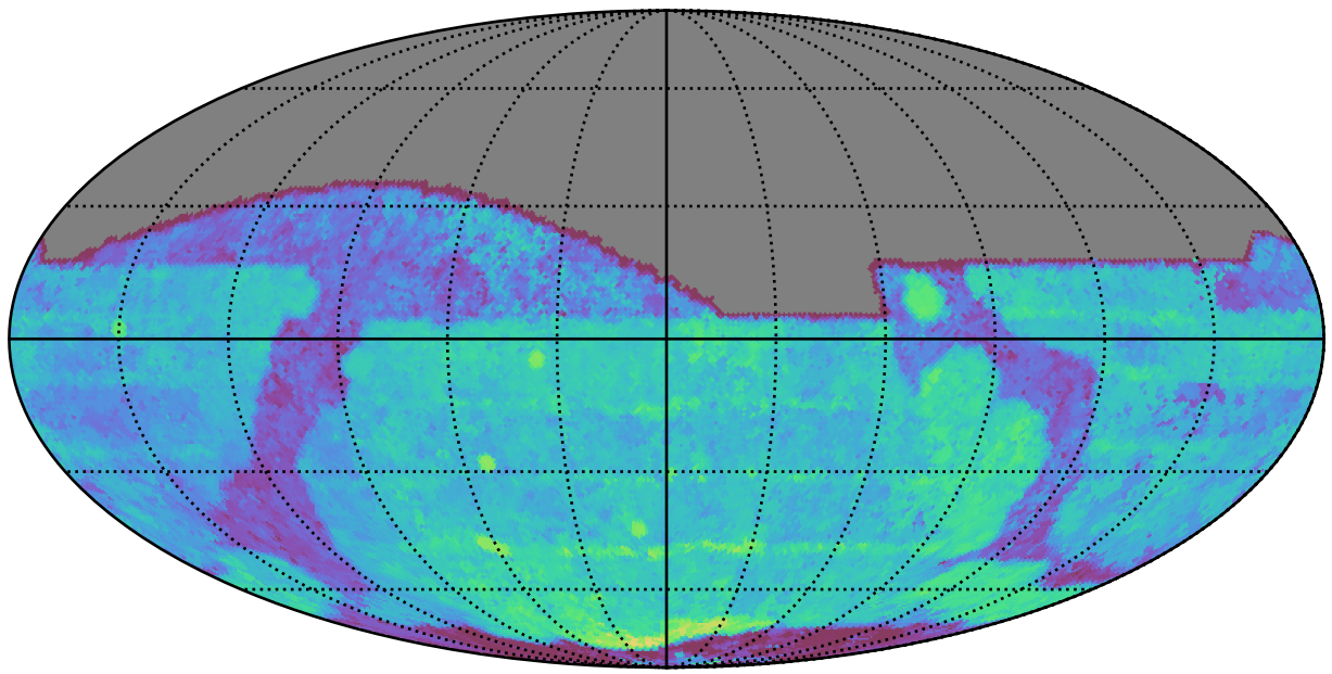
too_elab_2yr_r128_d3_ugrizy_v3.4_10yrs All sky i band: Median Season Length
