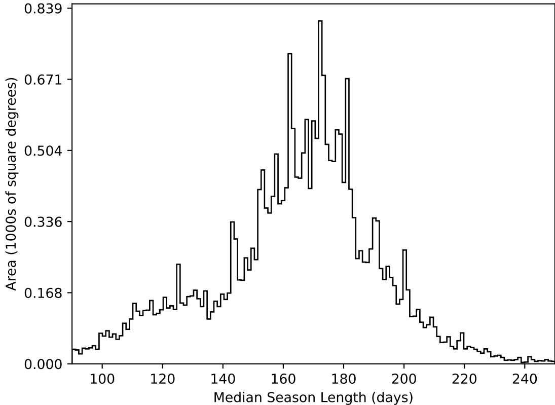
too_elab_2yr_r128_d3_ugrizy_v3.4_10yrs All sky all bands: Median Season Length
