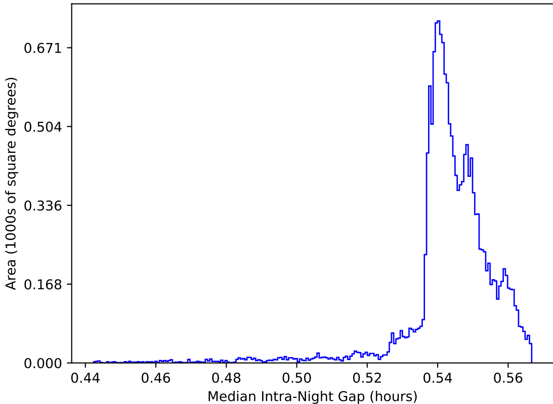
too_elab_2yr_r128_d3_ugrizy_v3.4_10yrs WFD: Median Intra-Night Gap
