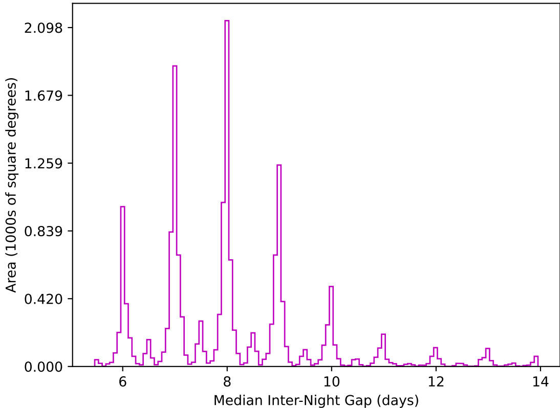
too_elab_2yr_r128_d3_ugrizy_v3.4_10yrs WFD z band: Median Inter-Night Gap
