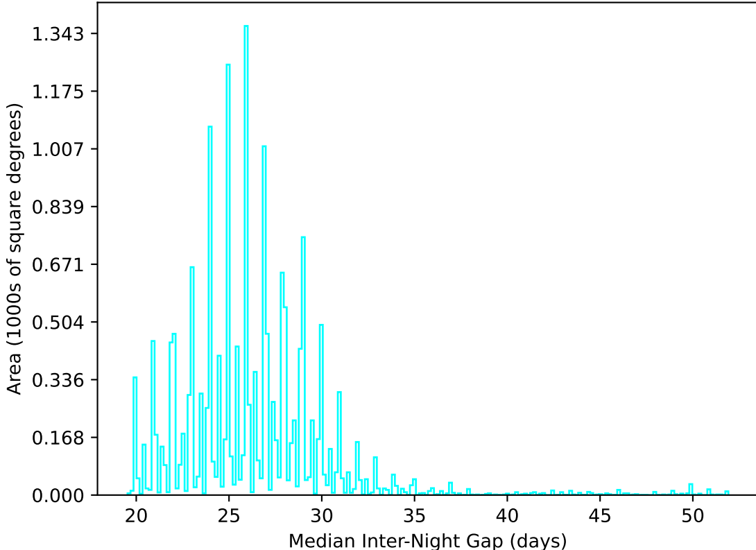
too_elab_2yr_r128_d3_ugrizy_v3.4_10yrs WFD u band: Median Inter-Night Gap
