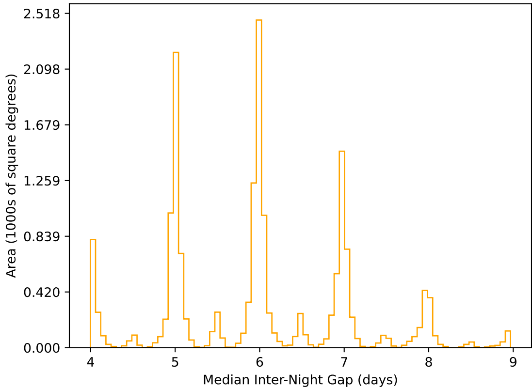
too_elab_2yr_r128_d3_ugrizyv3.4_10yrs WFD r band: Median Inter-Night Gap
