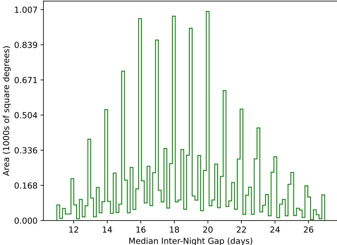
too_elab_2yr_r128_d3_ugrizy_v3.4_10yrs WFD g band: Median Inter-Night Gap
