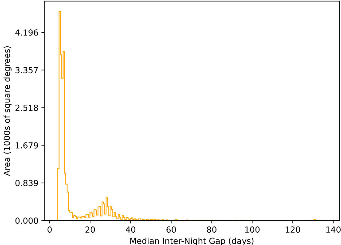
too_elab_2yr_r128_d3_ugrizy_v3.4_10yrs All sky r band: Median Inter-Night Gap
