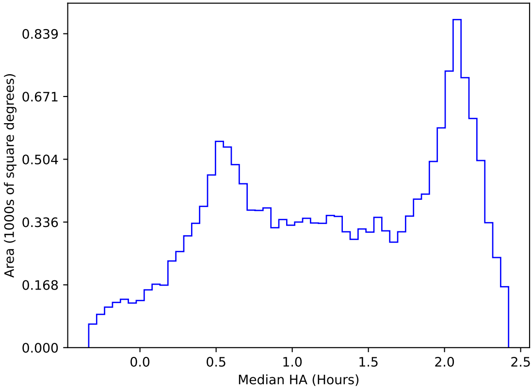
too_elab_2yr_r128_d3_ugrizy_v3.4_10yrs WFD y band: Median HA
