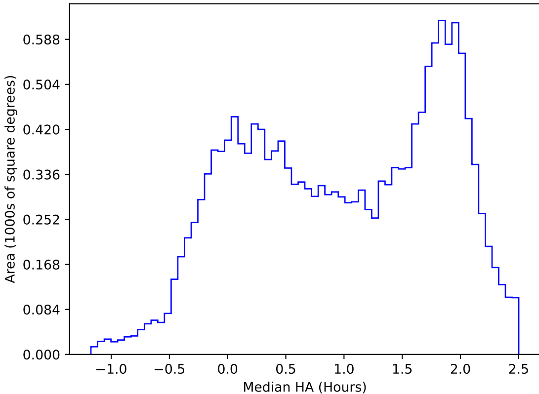
too_elab_2yr_r128_d3_ugrizy_v3.4_10yrs WFD u band: Median HA
