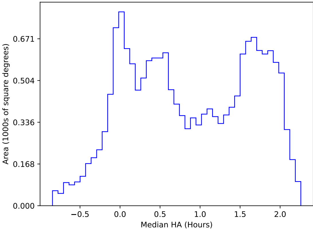
too_elab_2yr_r128_d3_ugrizy_v3.4_10yrs WFD r band: Median HA
