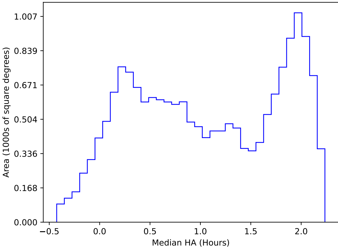
too_elab_2yr_r128_d3_ugrizy_v3.4_10yrs WFD i band: Median HA
