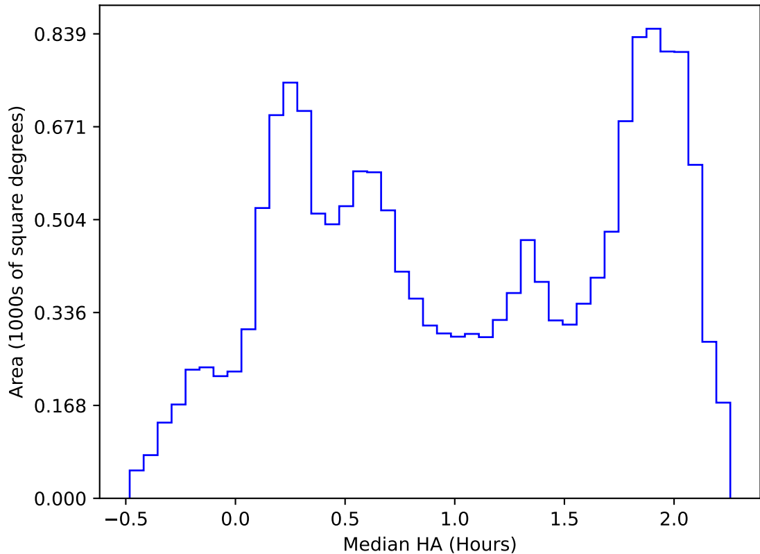
too_elab_2yr_r128_d3_ugrizy_v3.4_10yrs WFD all bands: Median HA
