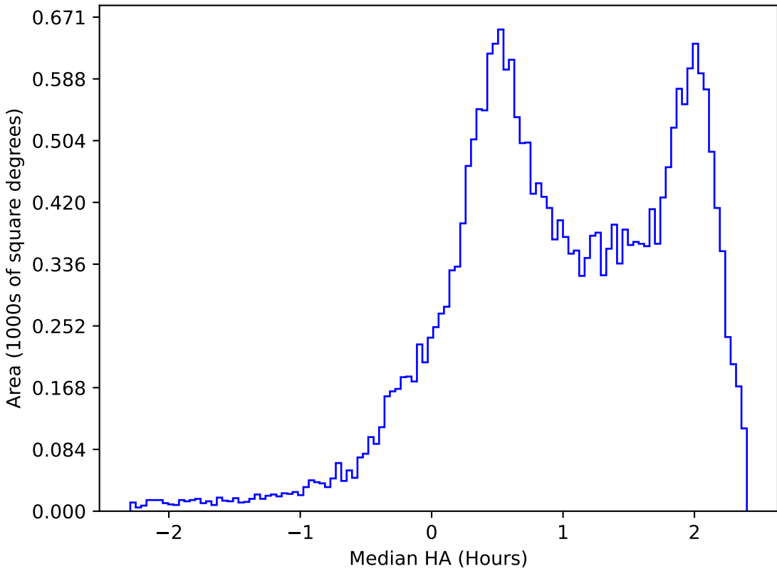
too_elab_2yr_r128_d3_ugrizy_v3.4_10yrs All sky z band: Median HA
