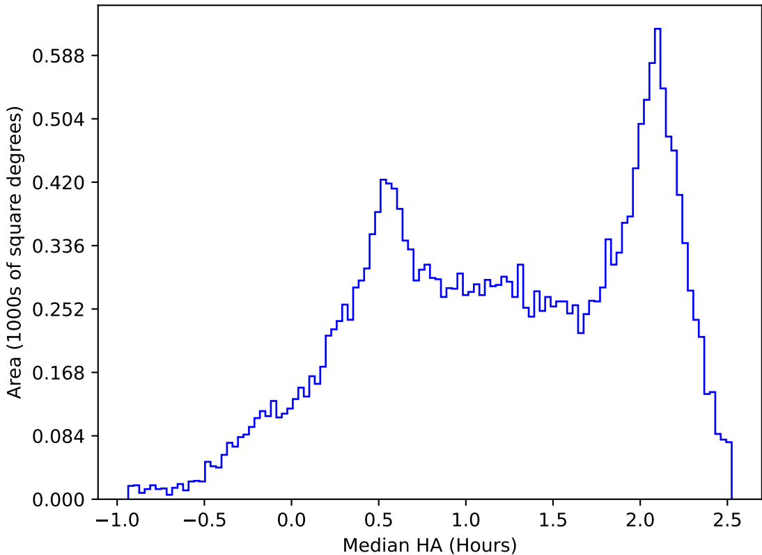
too_elab_2yr_r128_d3_ugrizy_v3.4_10yrs All sky y band: Median HA
