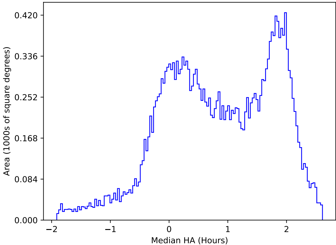
too_elab_2yr_r128_d3_ugrizy_v3.4_10yrs All sky u band: Median HA
