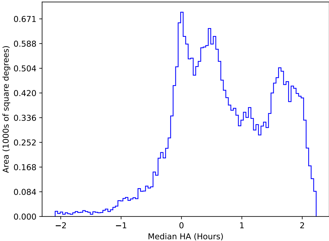
too_elab_2yr_r128_d3_ugrizy_v3.4_10yrs All sky r band: Median HA
