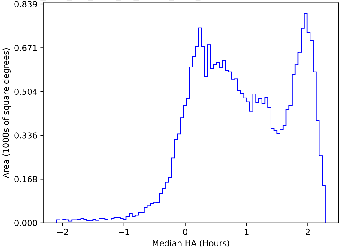
too_elab_2yr_r128_d3_ugrizy_v3.4_10yrs All sky i band: Median HA
