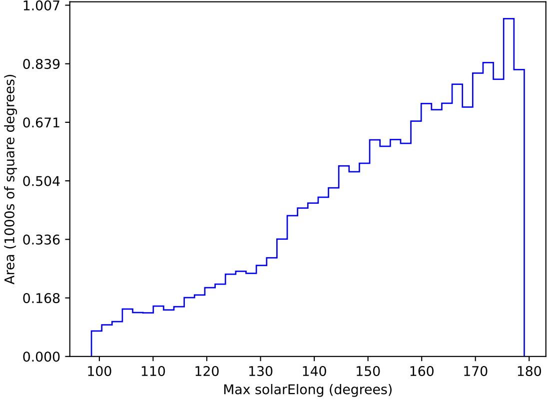
too_elab_2yr_r128_d3_ugrizy_v3.4_10yrs WFD g band: Max solarElong
