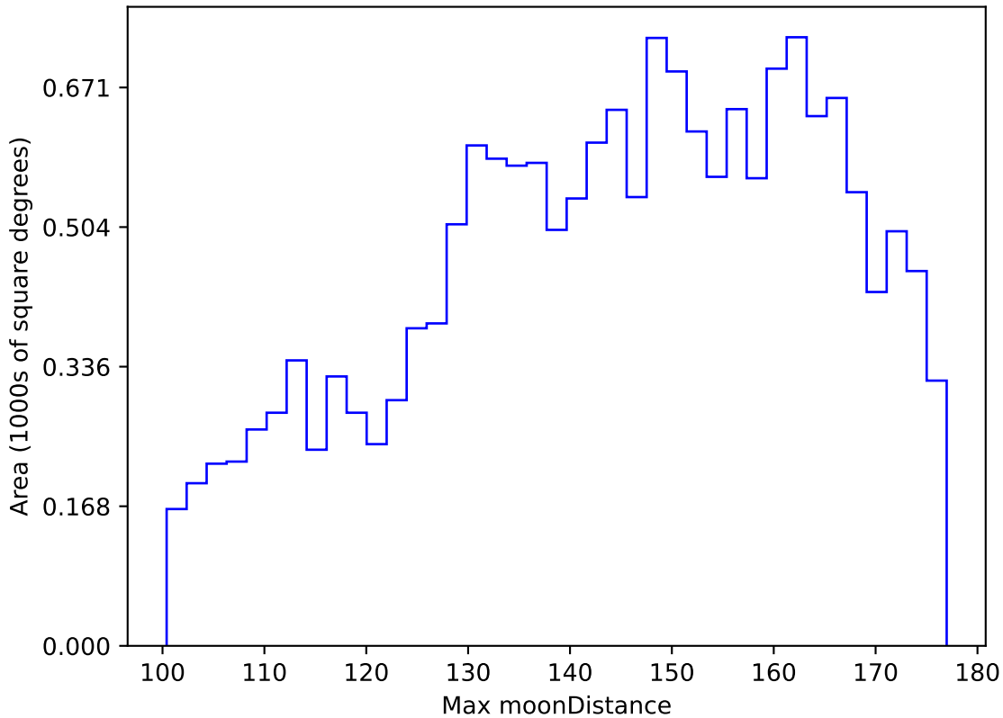
too_elab_2yr_r128_d3_ugrizy_v3.4_10yrs WFD y band: Max moonDistance
