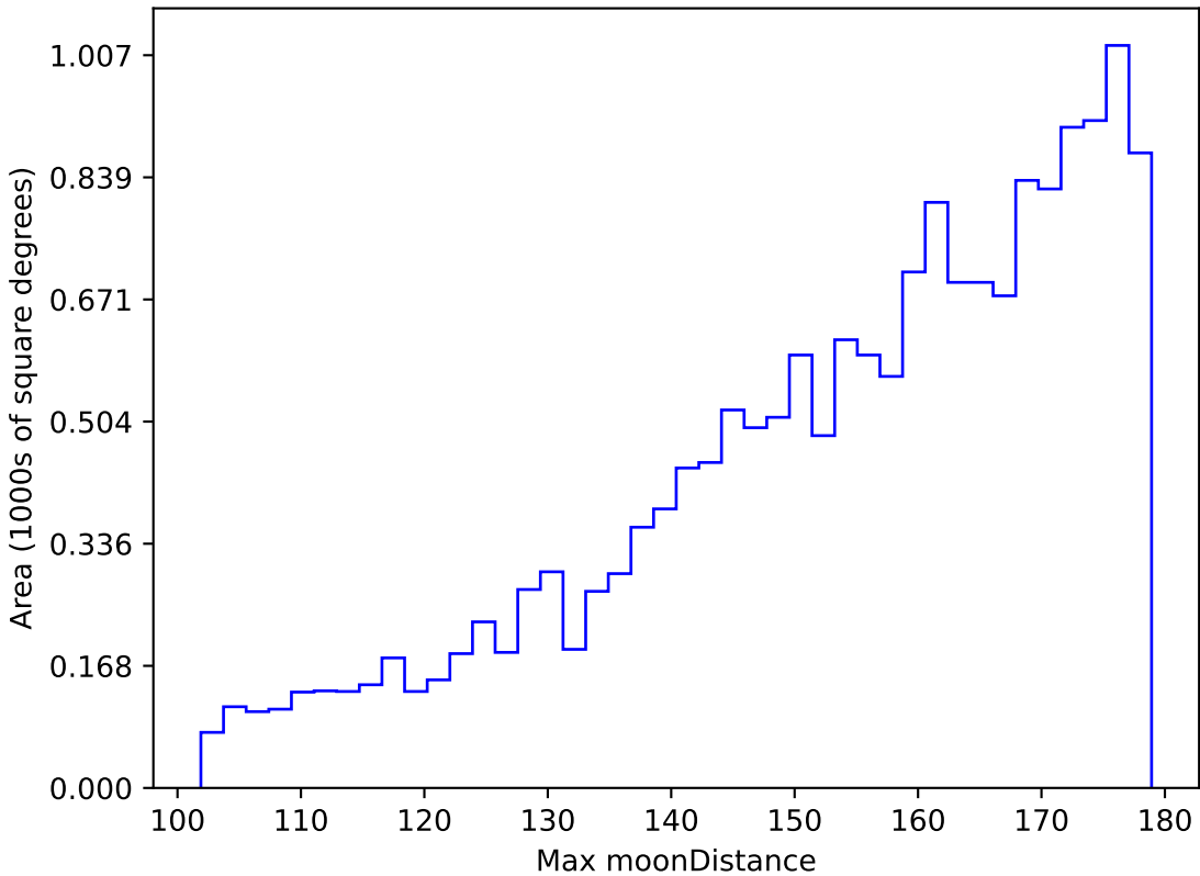
too_elab_2yr_r128_d3_ugrizy_v3.4_10yrs WFD u band: Max moonDistance
