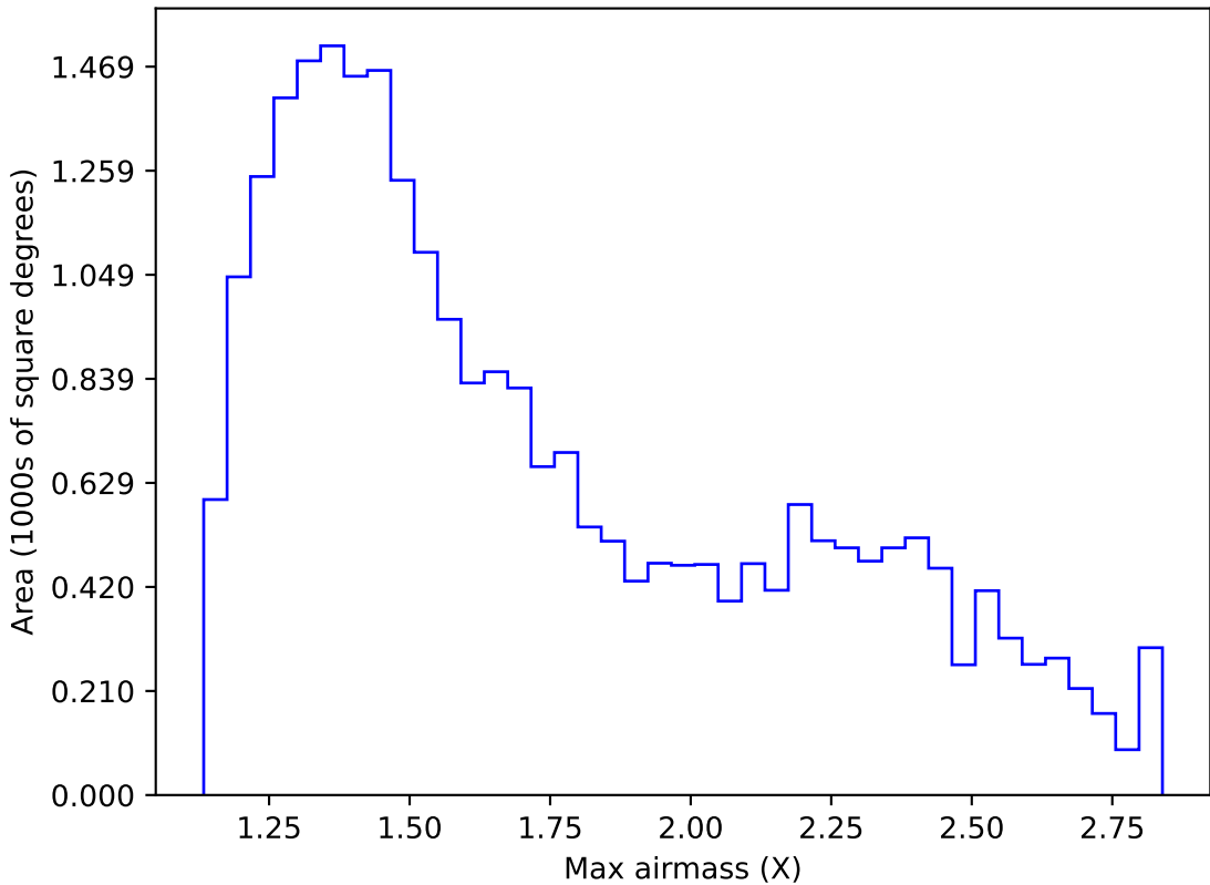
too_elab_2yr_r128_d3_ugrizy_v3.4_10yrs Yr 1 z band: Max airmass
