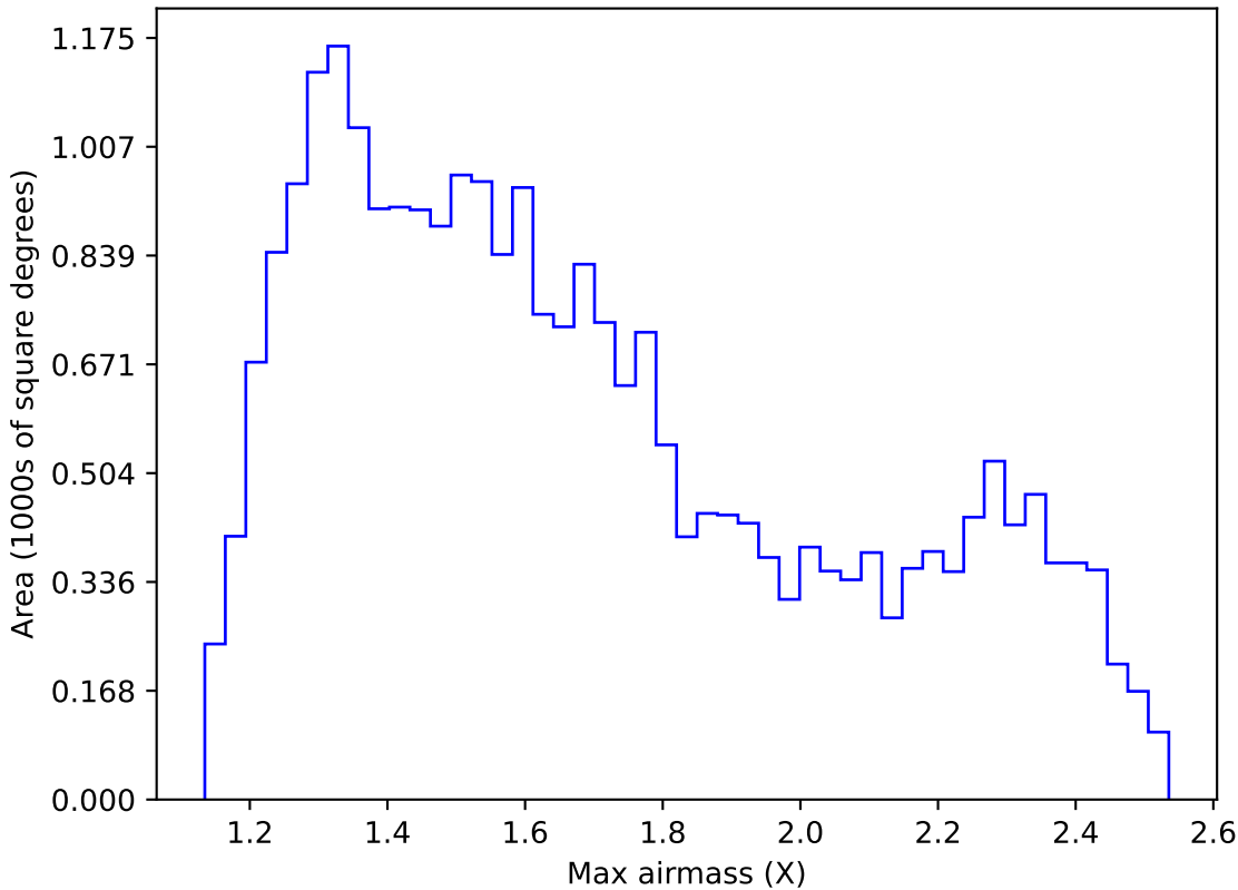
too_elab_2yr_r128_d3_ugrizy_v3.4_10yrs Yr 1 r band: Max airmass
