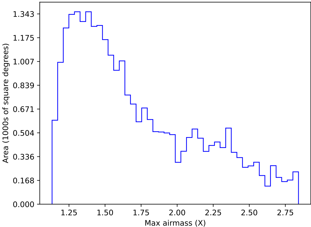
too_elab_2yr_r128_d3_ugrizy_v3.4_10yrs Yr 1 i band: Max airmass
