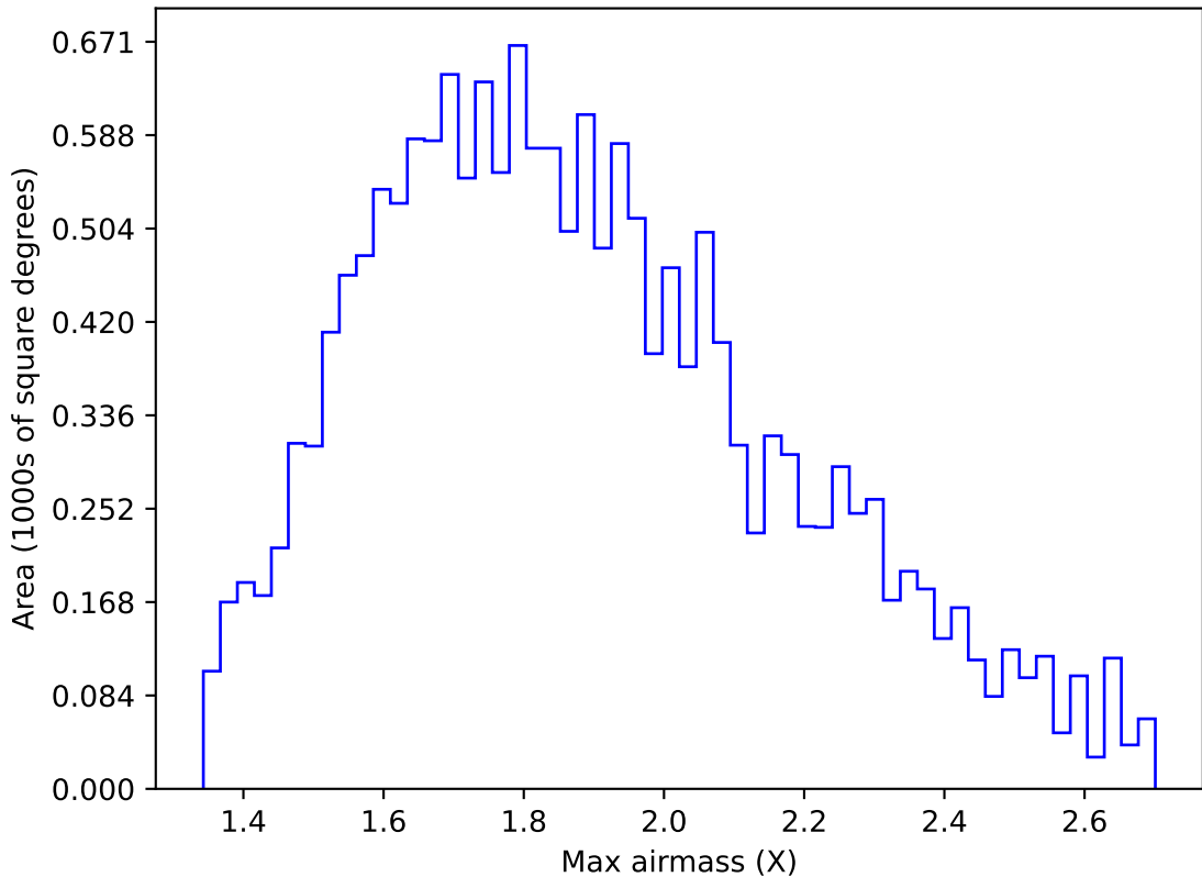
too_elab_2yr_r128_d3_ugrizy_v3.4_10yrs WFD u band: Max airmass
