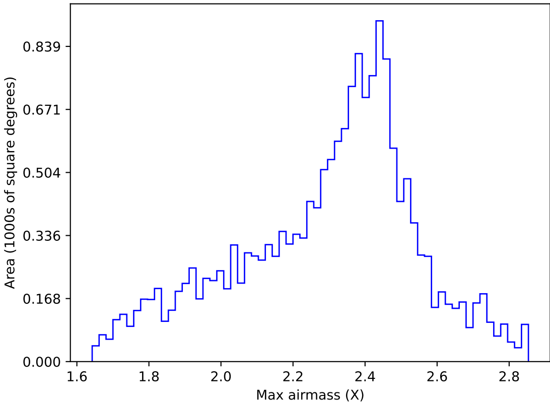
too_elab_2yr_r128_d3_ugrizy_v3.4_10yrs WFD r band: Max airmass
