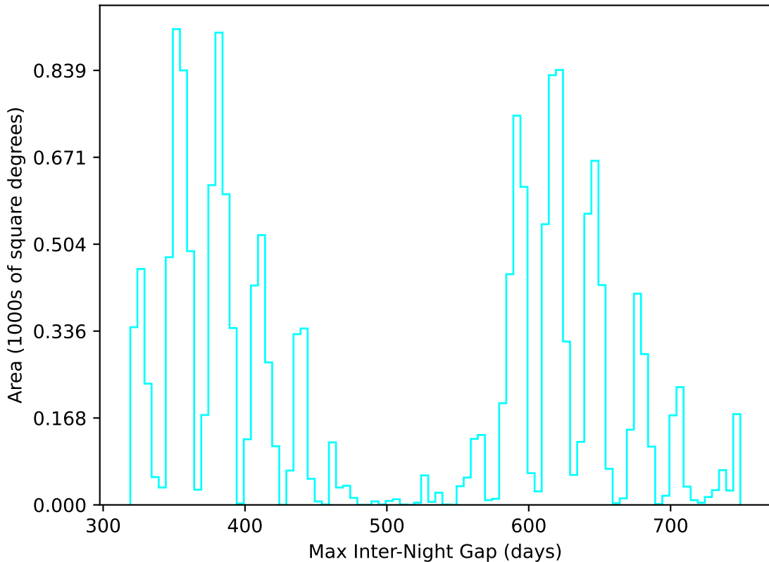
too_elab_2yr_r128_d3_ugrizy_v3.4_10yrs WFD u band: Max Inter-Night Gap
