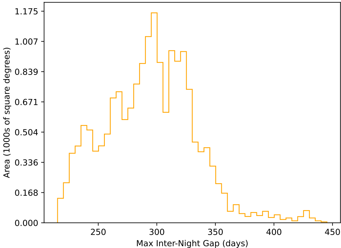
too_elab_2yr_r128_d3_ugrizy_v3.4_10yrs WFD r band: Max Inter-Night Gap
