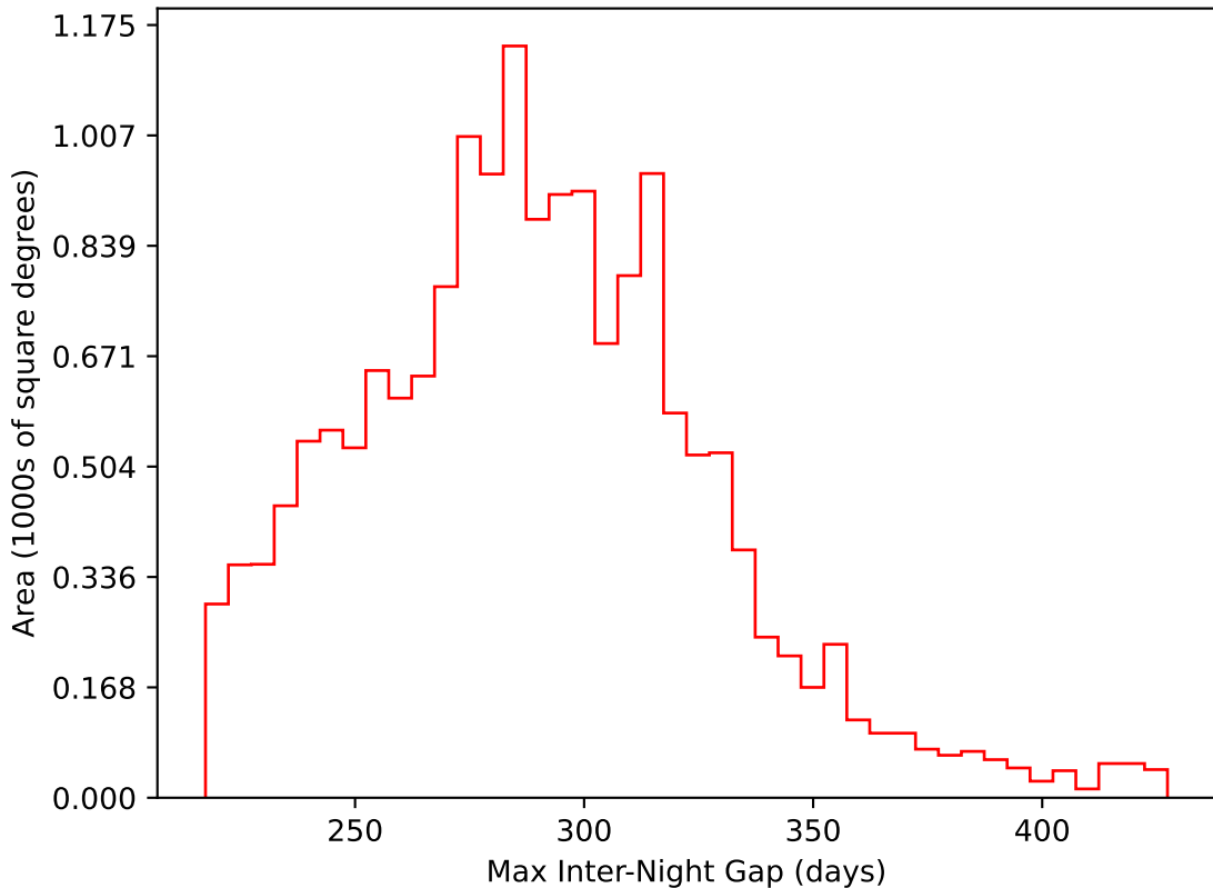
too_elab_2yr_r128_d3_ugrizy_v3.4_10yrs WFD i band: Max Inter-Night Gap
