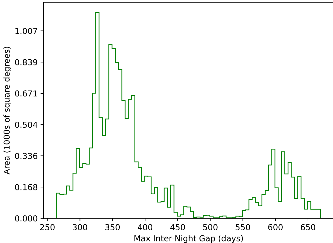
too_elab_2yr_r128_d3_ugrizy_v3.4_10yrs WFD g band: Max Inter-Night Gap
