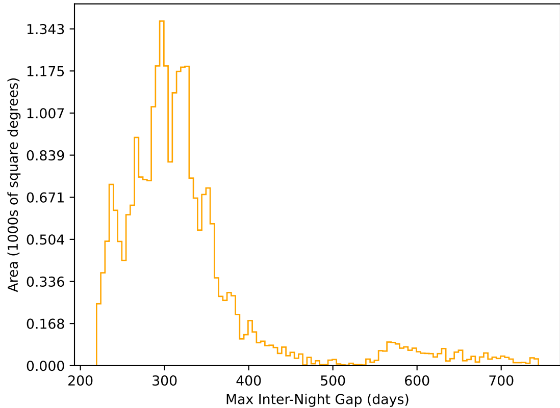
too_elab_2yr_r128_d3_ugrizy_v3.4_10yrs All sky r band: Max Inter-Night Gap
